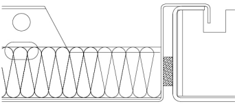
French hook
