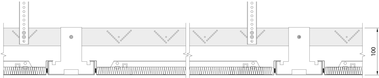
Section Drawing
